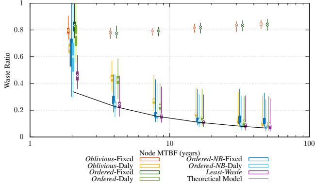
Fig. 3. Waste as a function of the system MTBF for the seven I/O and Checkpointing scheduling strategies.
