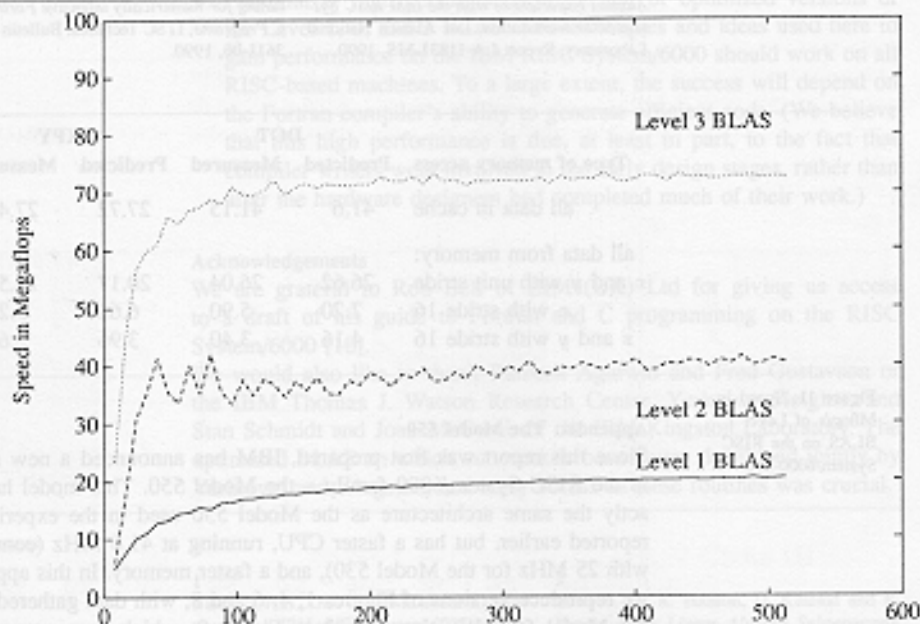
Figure 14. Speed of Level 1, 2, and 3 BLAS on the RISC System/6000-550.
