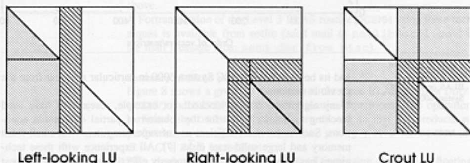
Figure 9. Variants of LU factorization on the RISC System/6000-530.
