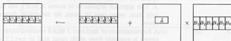
Partitioning of large matrix-matrix product
