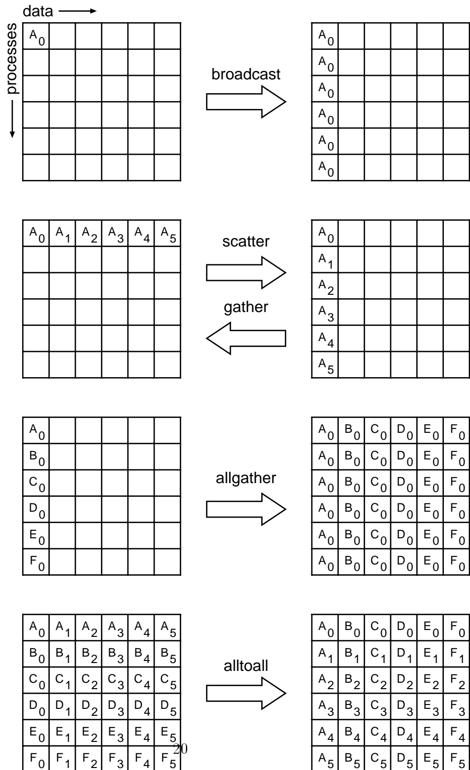
Figure 3: Collective move functions illustrated for a group of six processes. In each case, each row of boxes represents data locations in one process. Thus, in the broadcast, initially just the first process contains the data A_0 , but after the broadcast all processes contain it.
