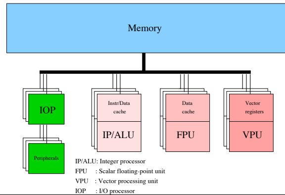
Figure 3.1. Blockdiagram of a vector processor.
