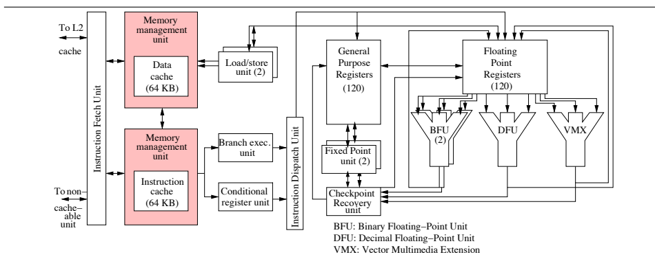
Figure 9.11. Block diagram of the IBM POWER6 core.
