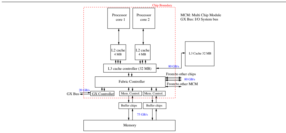
Figure 9.10. Diagram of the IBM POWER6 chip layout
