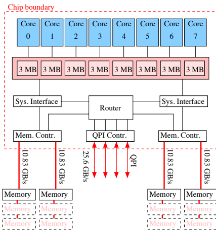
Figure 9.18. Diagram of a Nehalem EX processor.
