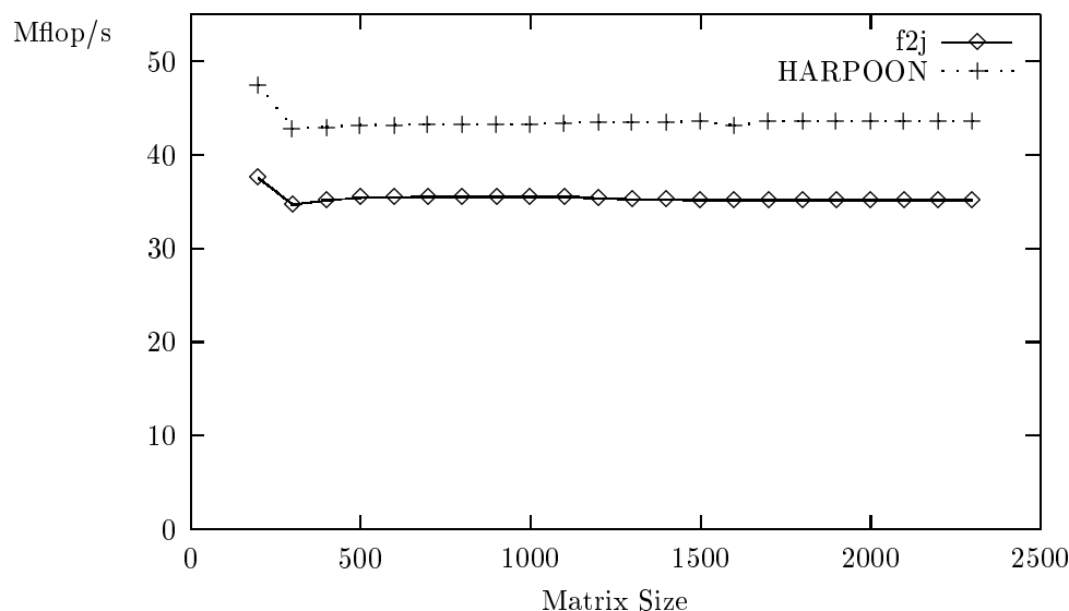
Figure 3: Comparison of f2j-generated DGEMM with Object-oriented Version
