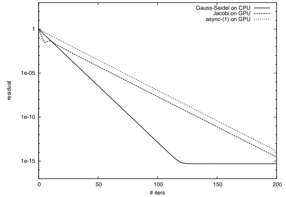
Fig. 5: Convergence behavior of test matrix FV1
