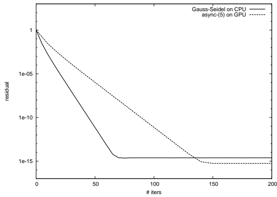
Fig. 10: Convergence behavior of async-(5) for test matrix CHEM97ZTZ
