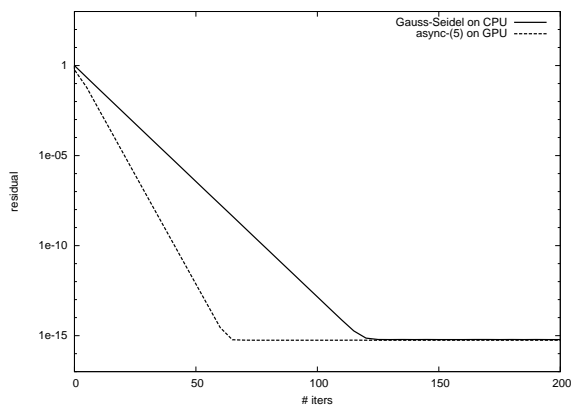
Fig. 12: Convergence behaviour of async-(5) for test matrix FV2
