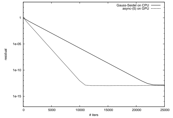
Fig. 13: Convergence behavior of async-(5) for test matrix FV3
