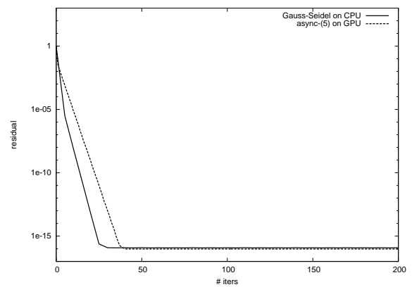
Fig. 15: Convergence behavior of async-(5) for test matrix TREFETHEN_2000
