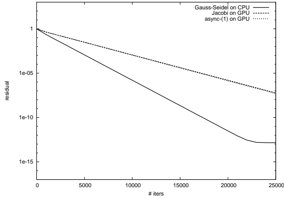
Fig. 7: Convergence behavior of test matrix FV3
