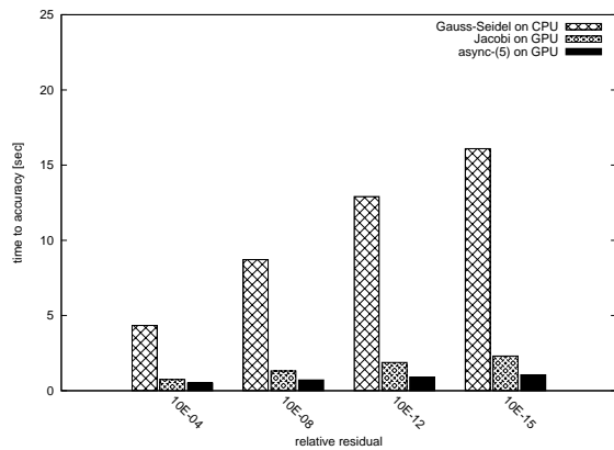
Fig. 18: Time to solution for FV1.
