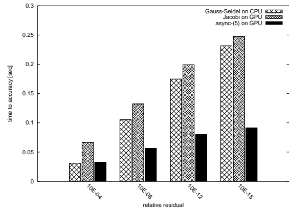
Fig. 21: Time to solution for TREFETHEN_2000.
