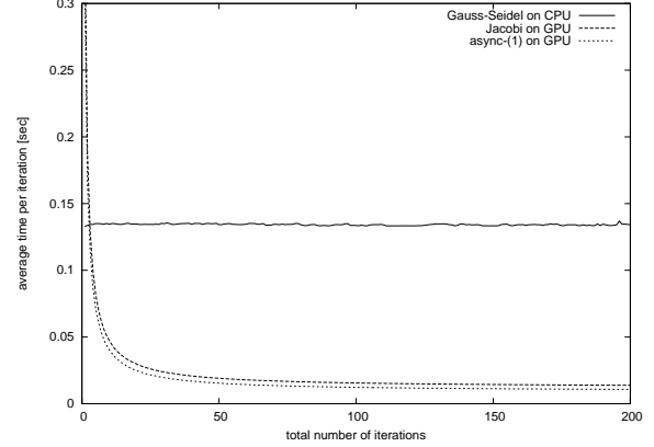
Fig. 16: Average iteration timings of CPU/GPU implementations depending on total iteration number, test matrix FV3.
