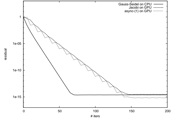
Fig. 4: Convergence behavior of test matrix CHEM97ZTZ
