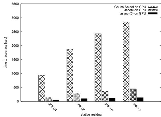
Fig. 20: Time to solution for FV3.
