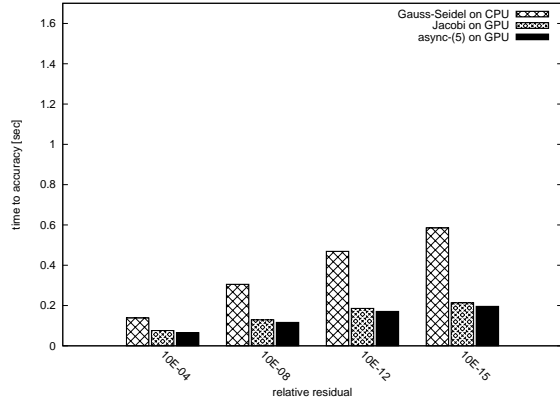
Fig. 17: Time to solution for CHEM97ZTZ.
