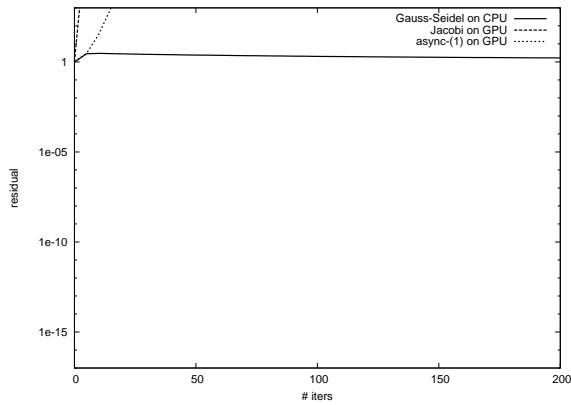
Fig. 8: Convergence behavior of test matrix S1RMT3M1
