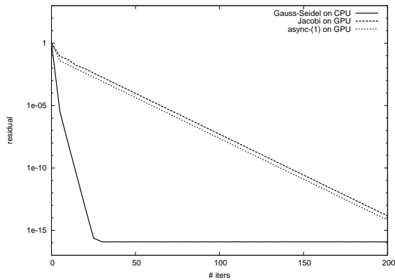
Fig. 9: Convergence behavior of test matrix TREFETHEN_2000
