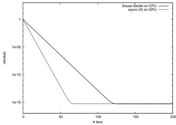
Fig. 11: Convergence behavior of async-(5) for test matrix FV1
