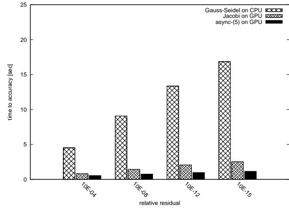
Fig. 19: Time to solution for FV2.
