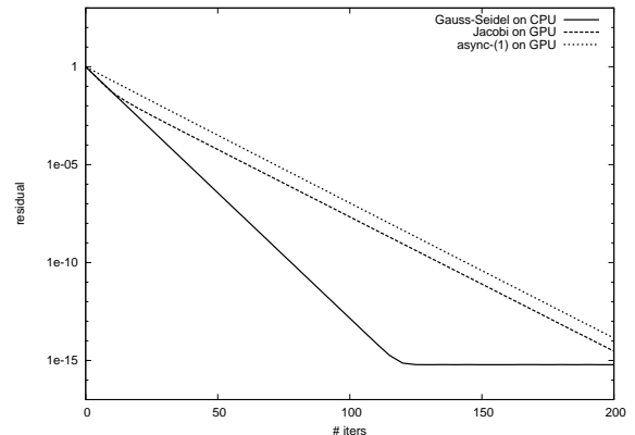
Fig. 6: Convergence behaviour of test matrix FV2
