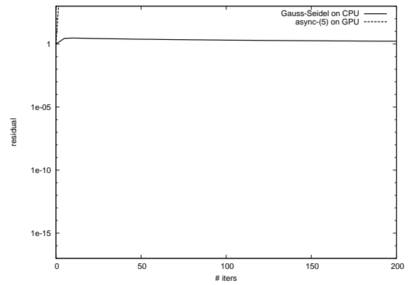
Fig. 14: Convergence behavior of async(5) for test matrix S1RMT3M1
