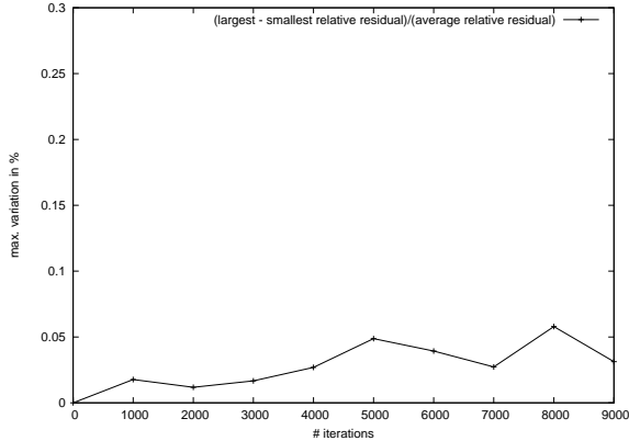
Fig. 3: Statistic convergence behaviour of asynchronous iteration method.
