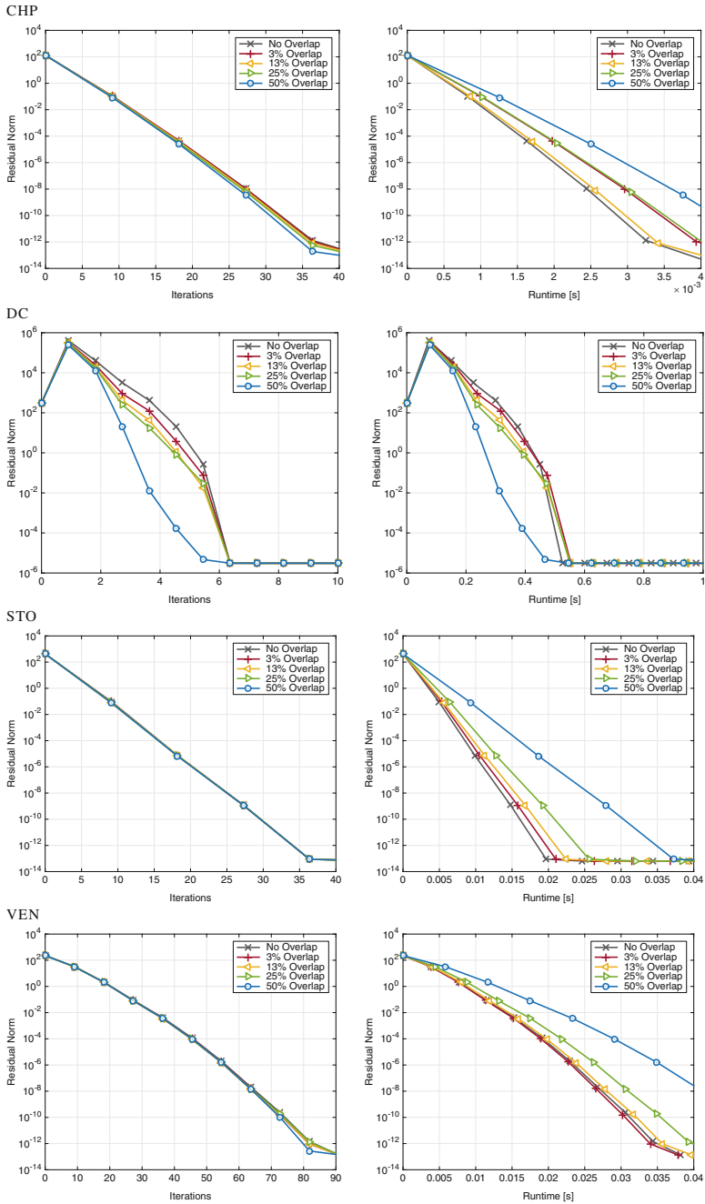
Fig. 8 Convergence (left) and residual-performance (right) of the block-asynchronous Jacobi using 2 Jacobi sweeps as local solver on the subdomains. The test cases are the sparse lower triangular systems arising as incomplete LU factorization without fill-in (ILU(0)) for the UFMC problems
