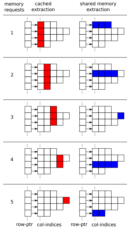
Figure 3. Illustration of the memory requests for the cached extraction and shared extraction (left and right, respectively). We assume warps of 4 threads, and visualize the data read by the distinct threads at each iteration with colored cells. We only show the accesses to the vector storing the col-indices of the CSR matrix structure; the access to the actual values induces far less overhead, as these memory locations are accessed only if a location belonging to a diagonal block is found. In that case, the access pattern is equivalent to the one used for col-indices.
