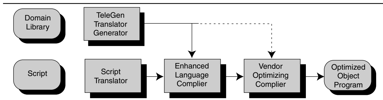
Fig. 2 Telescoping languages
