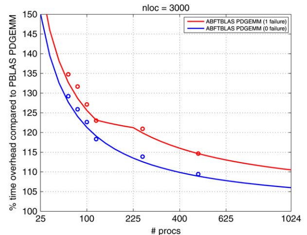
Fig. 6. Overhead of the fault tolerance with respect to the non-failure-resilient application PBLAS PDGEMM. The plain curves correspond to model while the circles correspond to experimental data. This is a weak scalability experiment with nloc = 3000 . (See also Table 2.)
