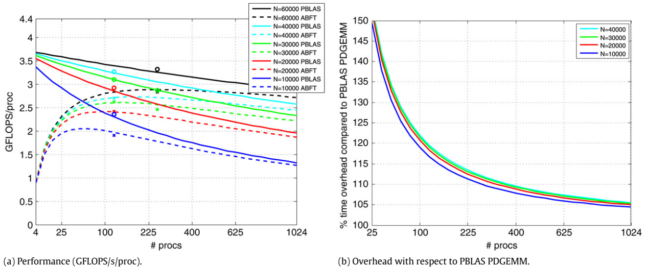
Fig. 7. Strong scalability of PBLAS PDGEMM and ABFT PDGEMM with 0 failure. On the left, performance for PBLAS PDGEMM (plain) and performance for ABFT PDGEMM (dashed). On the right, overhead of ABFT PDGEMM with respect to PBLAS PDGEMM.
