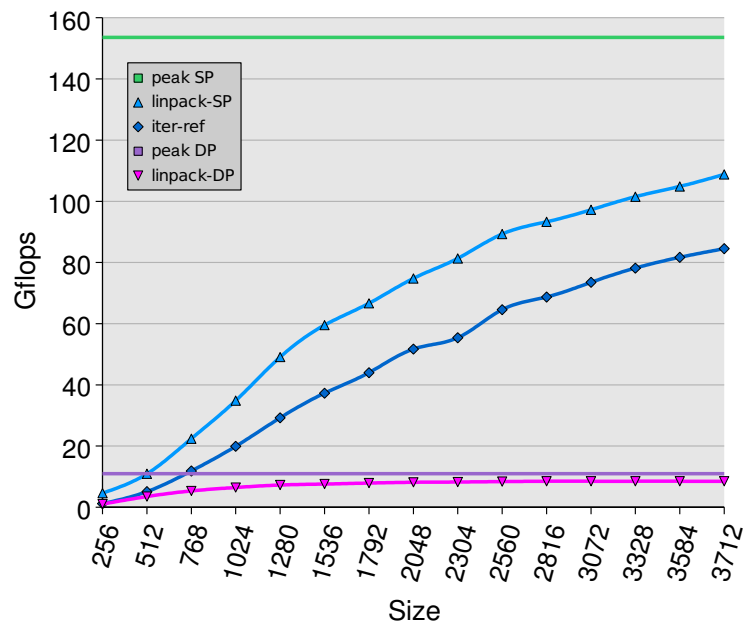
Figure 5. Performance comparison of solving linear system of equation A \times x = b on a 2.4 GHz Cell BE using the single-precision, double-precision and mixed-precision approach.
