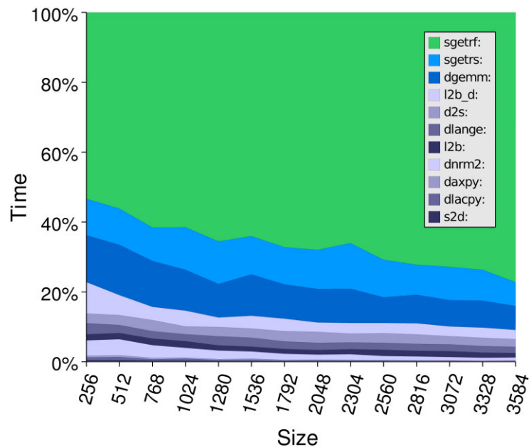
Figure 6. Breakdown of the execution time of solving linear system of equations using mixed-precision iterative refinement on a 2.4 GHz Cell BE.
