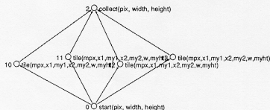
FIGURE 1 Simple HeNCE graph with dependency arcs.
