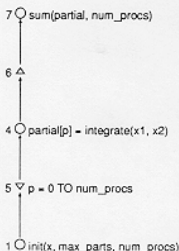
FIGURE 2 HeNCE program for numerical integration.
