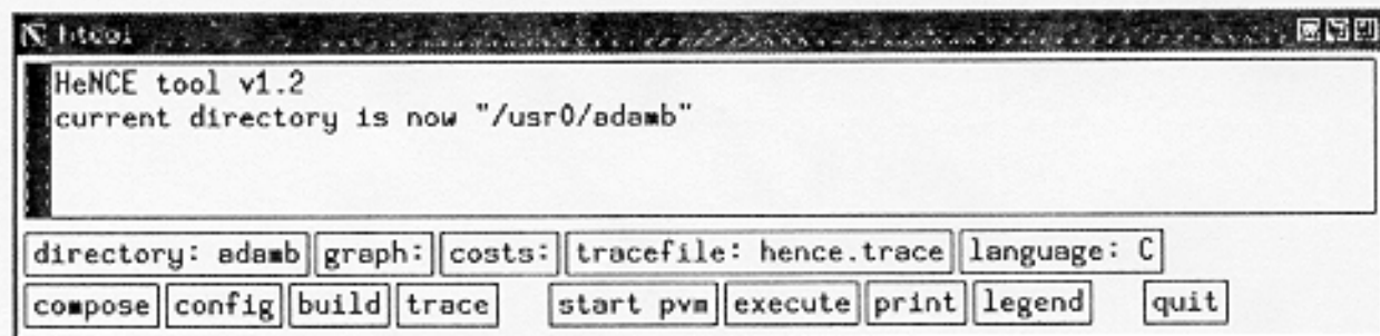
FIGURE 3 HeNCE main menu.
