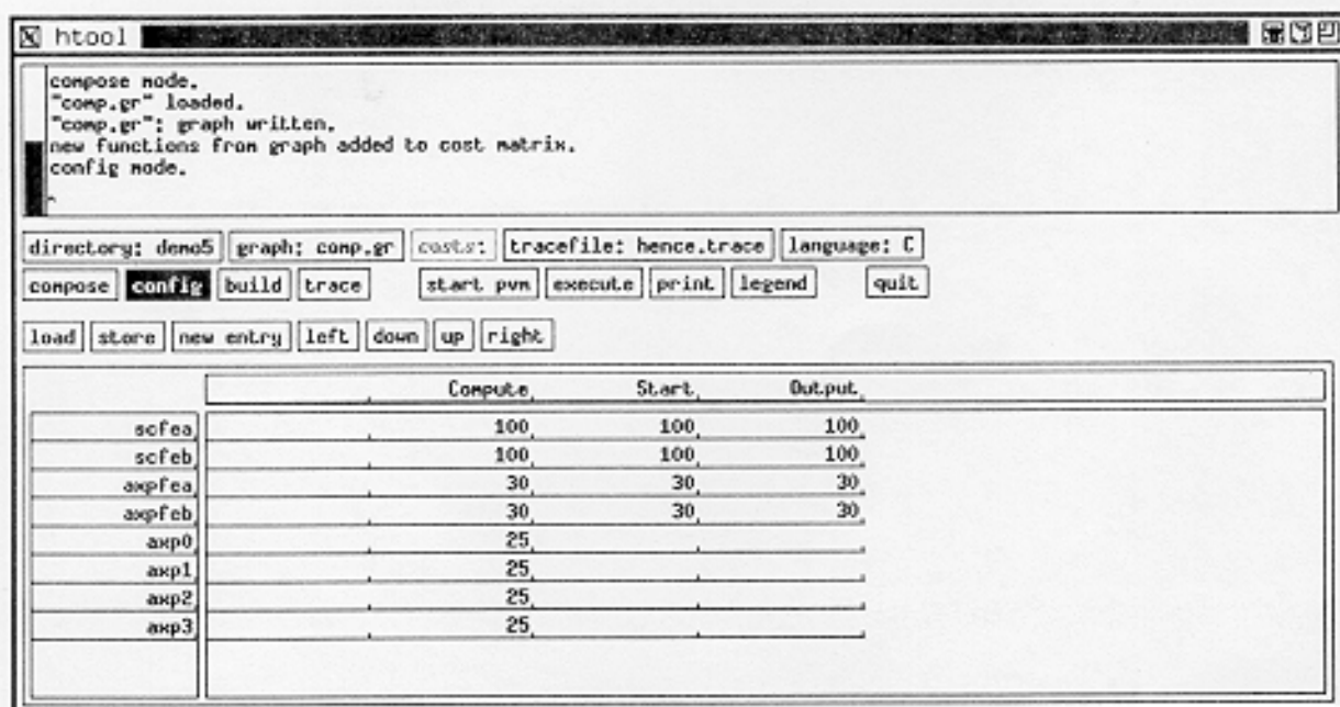
FIGURE 5 HeNCE in configure mode.
