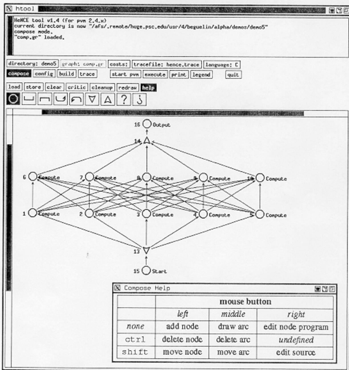
FIGURE 4 HeNCE in compose mode.
