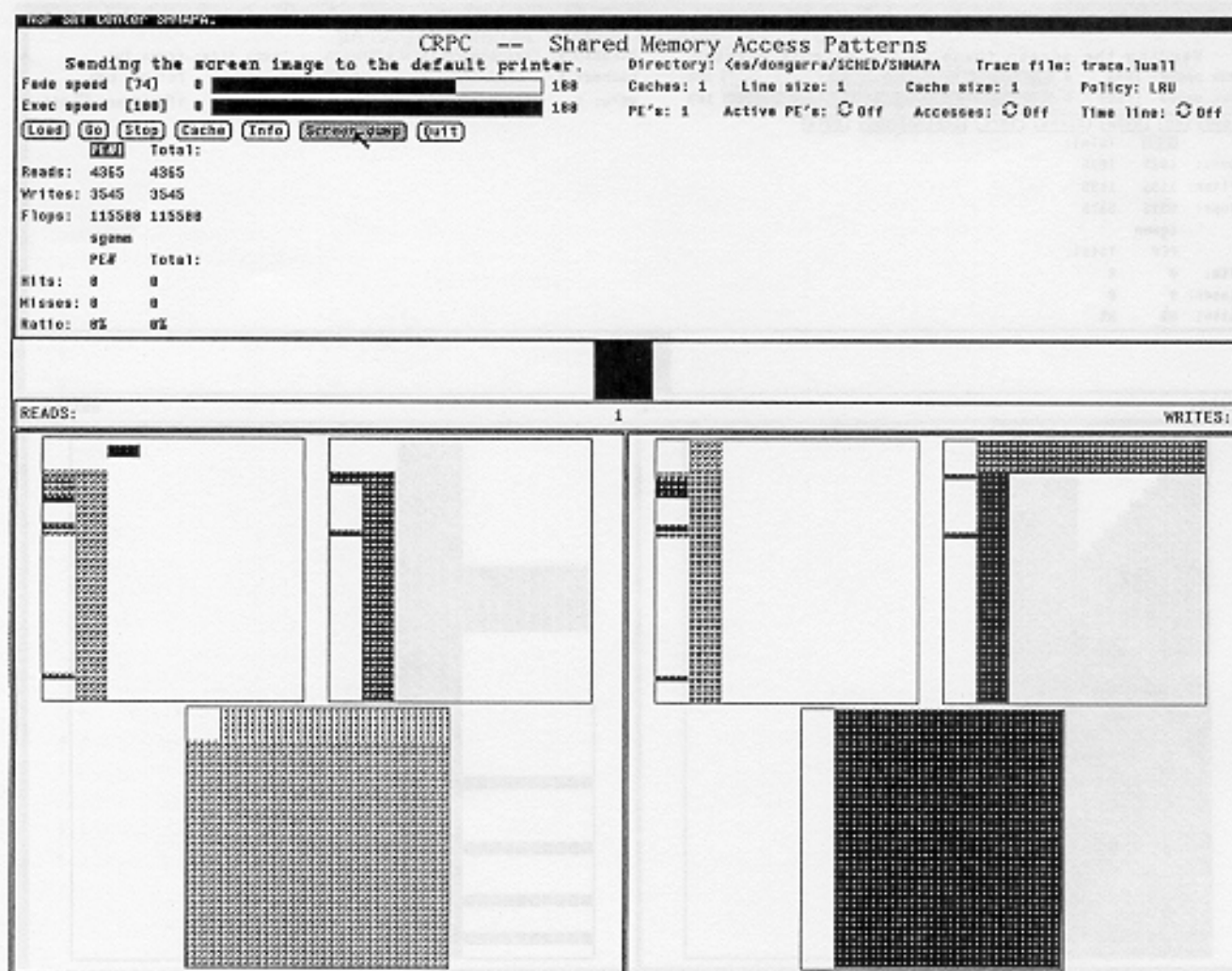
FIG. 2. Three algorithms performing LU decomposition.
