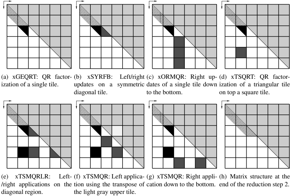
FIG. 4.4. Kernel execution breakdown of the TD&C algorithm during the first stage.
