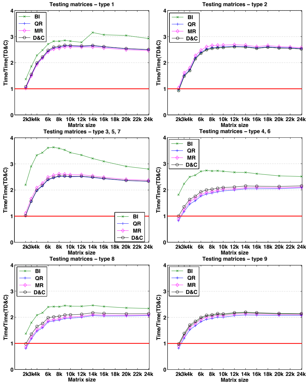
FIG. 6.5. TD&C Speed up as compared to BI, QR, MR, and D&C for all synthetic testing matrices from Table 6.1. For BI, QR, MR, and D&C, the MKL SBR-implementation routine DSYRDD is used to transform the dense symmetric matrix A to tridiagonal.
