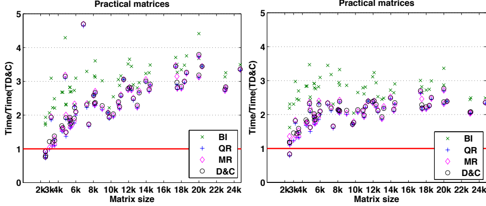
FIG. 6.6. Timings comparison for practical matrices. The tridiagonalisation has been done either by the MKL-LAPACK-DSYTRD (left) or by the MKL-SBR-DSYRDD (right).
