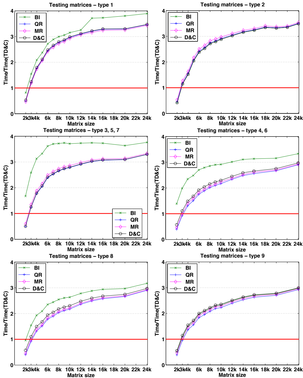
FIG. 6.4. TD&C Speed up as compared to BI, QR, MR, and D&C for all synthetic testing matrices from Table 6.1. For BI, QR, MR, and D&C, the MKL LAPACK-implementation routine DSYTRD is used to transform the dense symmetric matrix A to tridiagonal.
