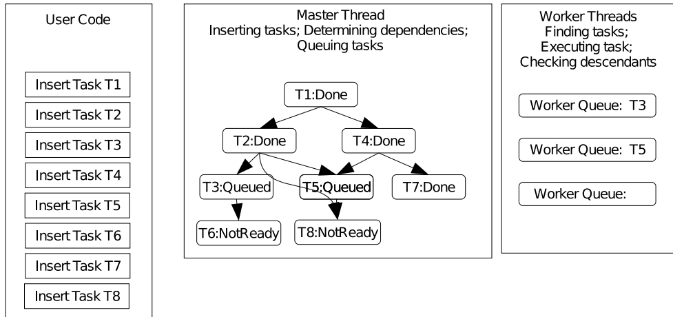
FIG. 4.3. Idealized architecture diagram for the dynamic scheduler. Inserted tasks go into a (implicit) DAG based on their dependencies. Tasks can be in NotReady, Queued or Done states. Workers execute queued tasks and then determine if any descendants have now become ready and can be queued.
