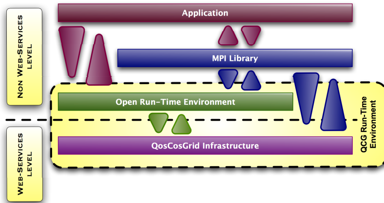
(a) Architecture of a QCG-OMPI application: communication library and run-time environment.
