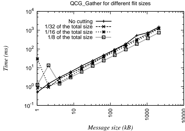
Fig. 4. Effects of message pre-cutting on QCG_Gather
