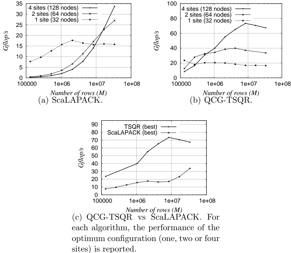
Fig. 9. Performance of QCG-TSQR and ScaLAPACK with a matrix of width N = 64 .
