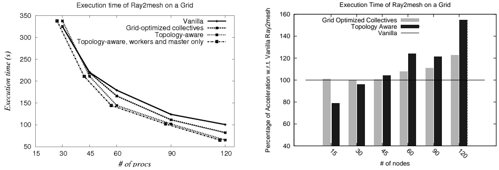
(a) Scalability of Ray2mesh on a grid (b) Relative acceleration of Ray2mesh, with respect to the vanilla implementation
