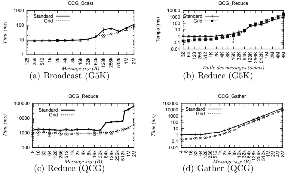
Fig. 5. Comparison between standard and grid-enabled collective operations on a grid.
