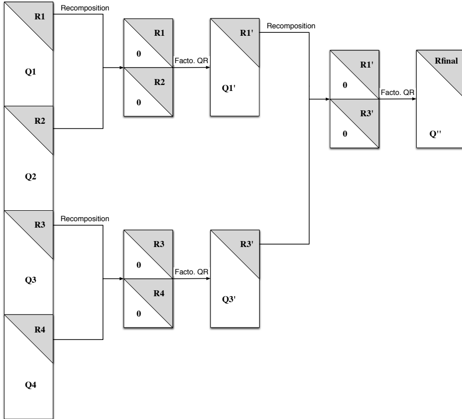
Fig. 8. TSQR algorithm. The initial tall and skinny matrix is split into four domains factorized independently from one another (left). The upper triangular matrices ( R_i ) are then assembled by pairs and factorized following a binary tree reduction (middle) until the final triangular factor R_{final} is obtained (right).
