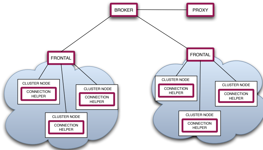
(b) Architecture of the grid infrastructure of QCG-OMPI.
