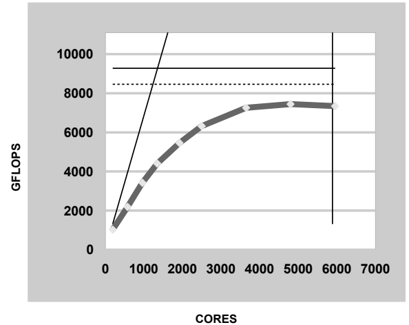
Figure 12. Systolic QR performance for a problem of size 20K \times 20K for tile size 192 and its theoretical performance bounds.
