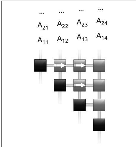
Figure 4. Data bypass in QR systolic array.
