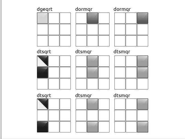
Figure 2. Kernel invocations in a 3 \times 3 tile QR.
