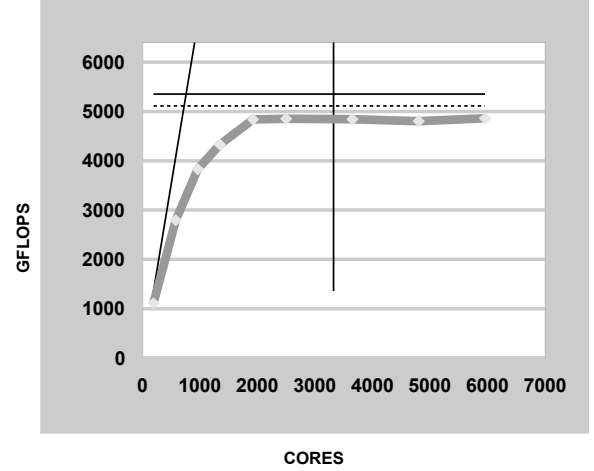
Figure 15. Systolic QR performance for a problem of size 20K \times 20K for tile size 256 and its theoretical performance bounds.
