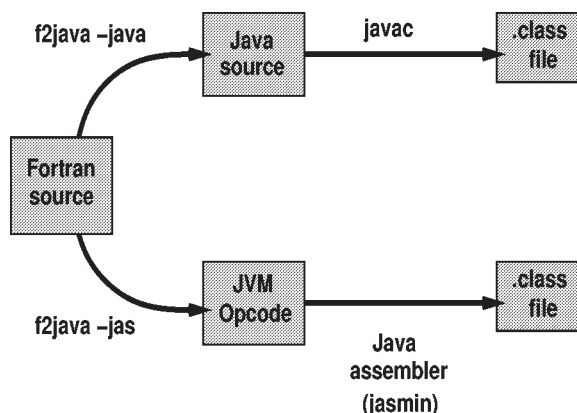
Fig. 2. Translation strategies in the f2j project.
