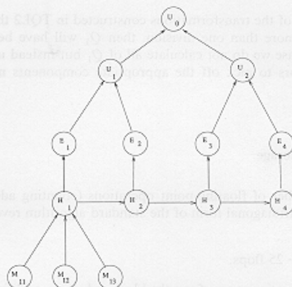
Fig. 2. Large-grain control flow graph.
