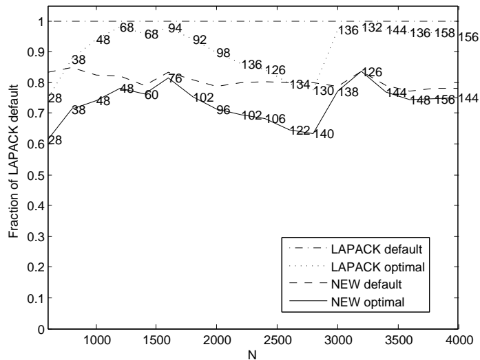
Figure 12: Execution times of the current LAPACK implementation and our new implementation using the default and optimal number of shifts. The execution times are given relative to LAPACK with the default number of shifts. Results from Abisko .
