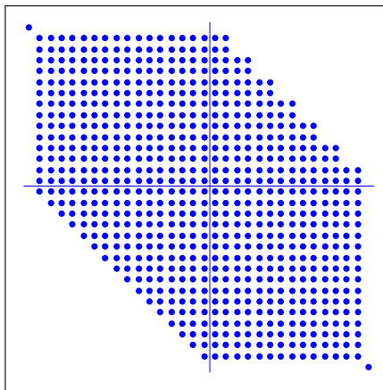
Figure 10: Typical nonzero pattern of the orthogonal transformation matrix for an optimally packed chain with m=2 , n_b=7 , and k=mn_b+2=16 (optimal).
