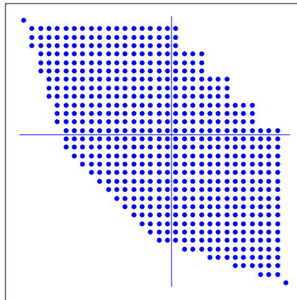
Figure 7: Sparsity pattern of the accumulated transformation matrix U for a tightly packed chain with m = 2 , n_b = 5 , and k = (m + 1)n_b + 1 = 16 (optimal).
