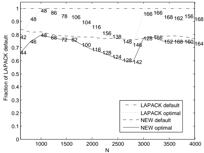
Figure 11: Execution times of the current LAPACK implementation and our new implementation using the default and optimal number of shifts. The execution times are given relative to LAPACK with the default number of shifts. Results from Akka .
