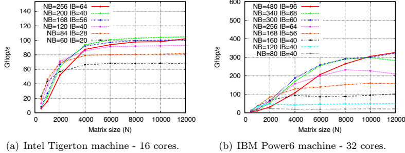
Figure 3: Performance of the PLASMA QR factorization
