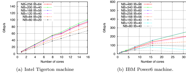
Figure 6: Strong scalability - N = 6000 .
