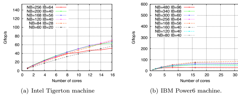
Figure 7: Strong scalability - N = 2000 .
