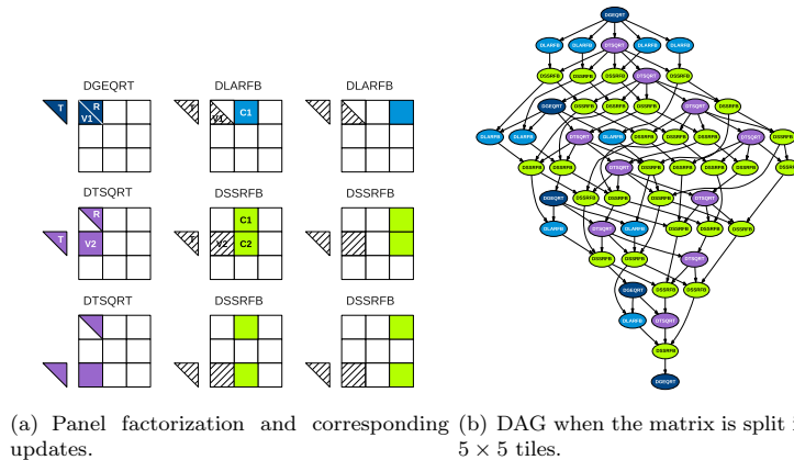
Figure 1: Tile QR Factorization
