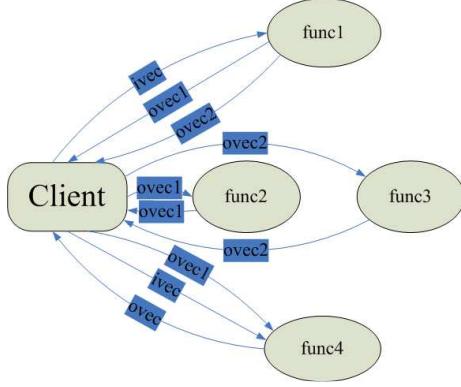
Fig. 2. An example of the standard data flow in GridSolve.
